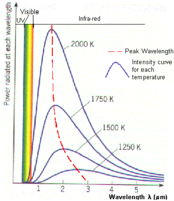
Fig: Black body radiation
