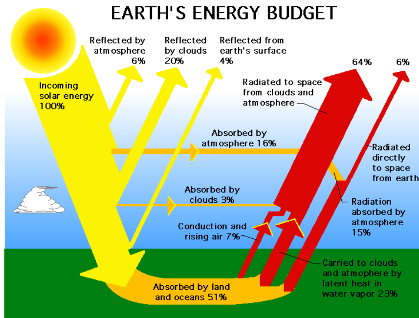
Fig: The Earth Radiation Budget is the balance between incoming energy from the sun and the outgoing longwave(thermal) and reflected shortwave energy from the Earth.
