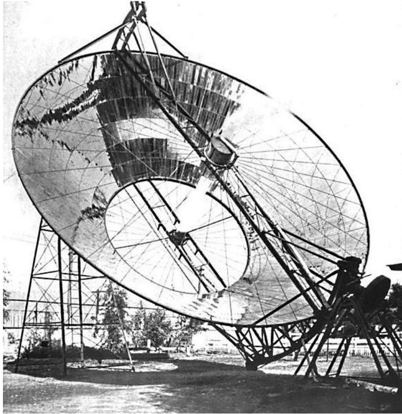
Fig. : 1901 "solar motor" in operation in California.
