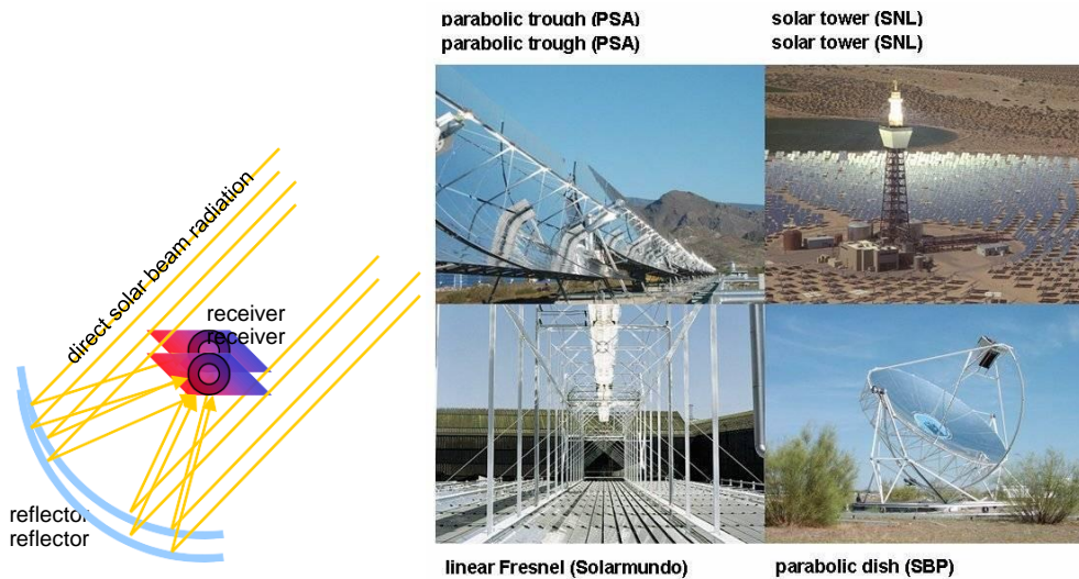
Fig: Principle of concentrating solar beam radiation and the four CSP collector technology main streams realized up to date
