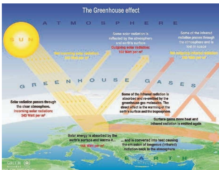
Fig: The greenhouse effect
