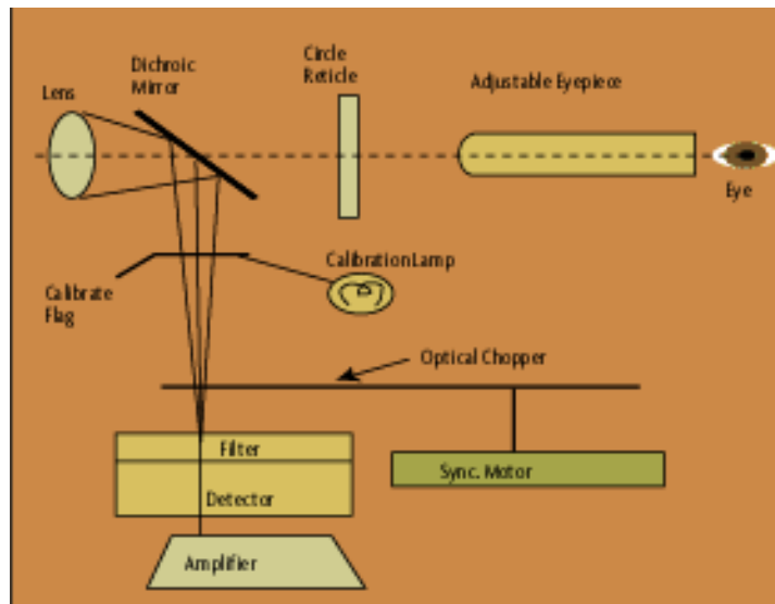
Fig: Automatic optical pyrometer
