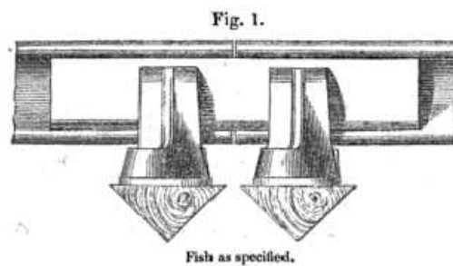
The first railway fishplate
