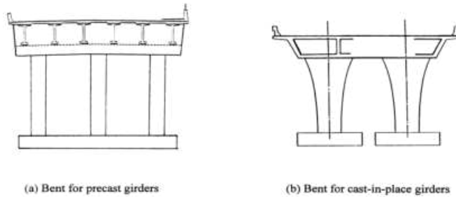
(a) Bent for precast girders
