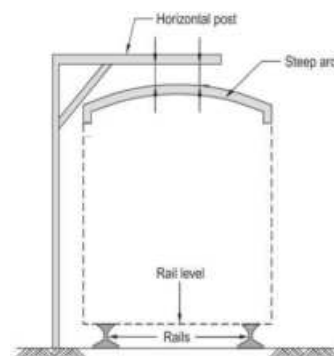
Fig. 2.2 Loading gauge
