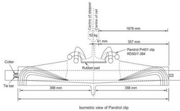
Isometric view of Pandrol clip
