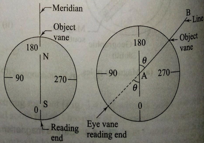
(c) Reading of a bearing
