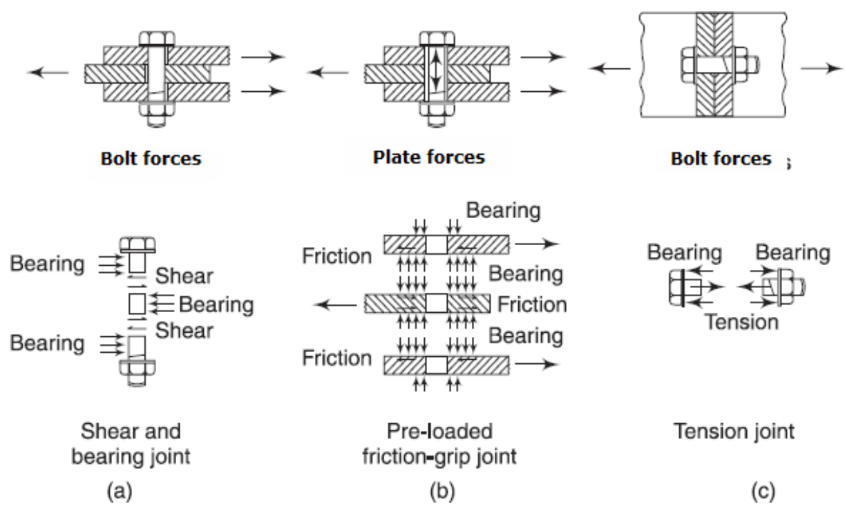
Figure 10.13 Force transmission through bolts
