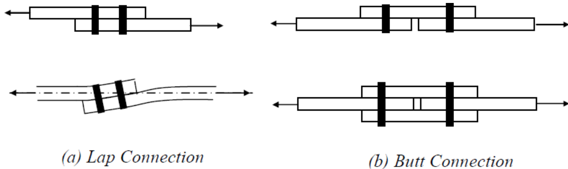
Figure 10.3 Shear connections
