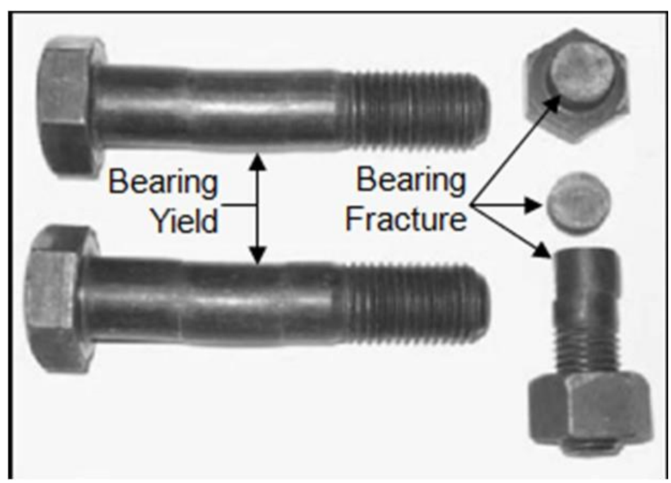
Figure 10.14 Bearing failure of bolts
